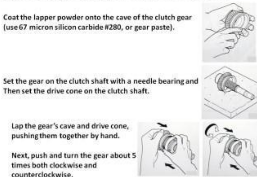
Figure 11: Step 7 Lapping Procedure For Drive Cone
